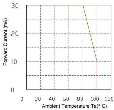
Derating
