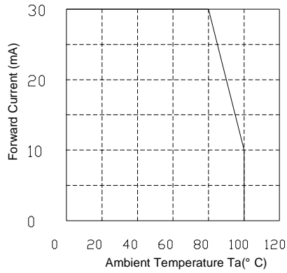
Derating
