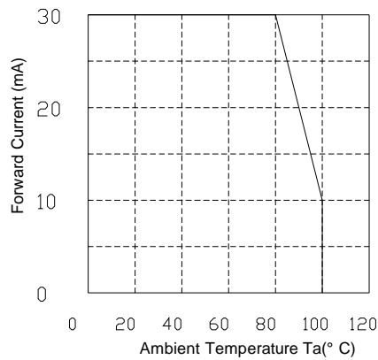
Derating
