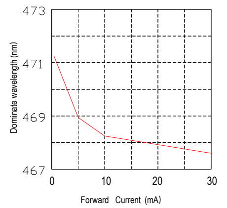
Forward Current vs. Dominate wavelength (Ta=25°C)
